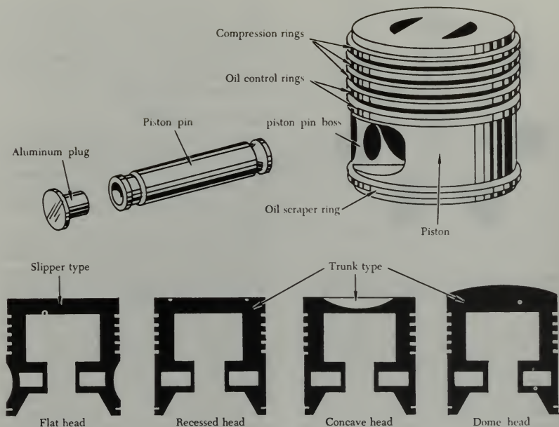
FIGURE 1-13. Piston assembly and types of pistons.
